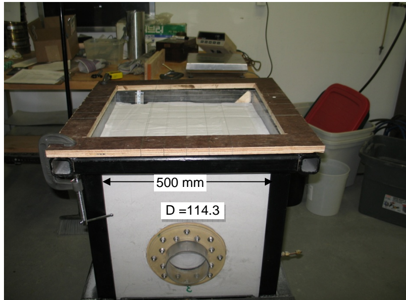
Figure 4. Experimental Set Up for Surface Soil Failure
